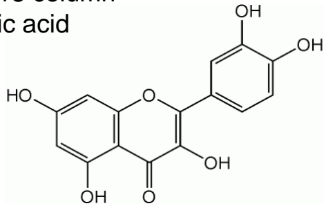
Quercetin
